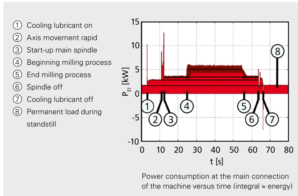
Figure 2: Process power and power consumption of a machine (source: ISW)
